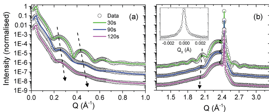
Fig. 3 Panel (a) shows X-ray reflectivity data and panel (b) shows high angle diffraction data, measured at exposure times of 30 s, 90 s and 120 s; the experimental data are represented by the open black circles and the fitted calculations by the solid green, blue and magenta lines, respectively. The insert of panel (b) shows the rocking curve of the (002) Bragg peak for the 30 s exposure. The dashed black arrows indicate an increase in fringe separation as a function of exposure time, which suggests a concomitant loss of material.
